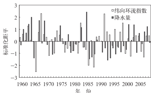
图 2 1960—2009 年 9 月陕西北部降水量标准化距平与纬向环流指数标准化距平比较 Fig. 2 The comparison between standard departure values of in Northern Shaanxi September rainfall and that of zonal circulation Index from 1960 to 2009
