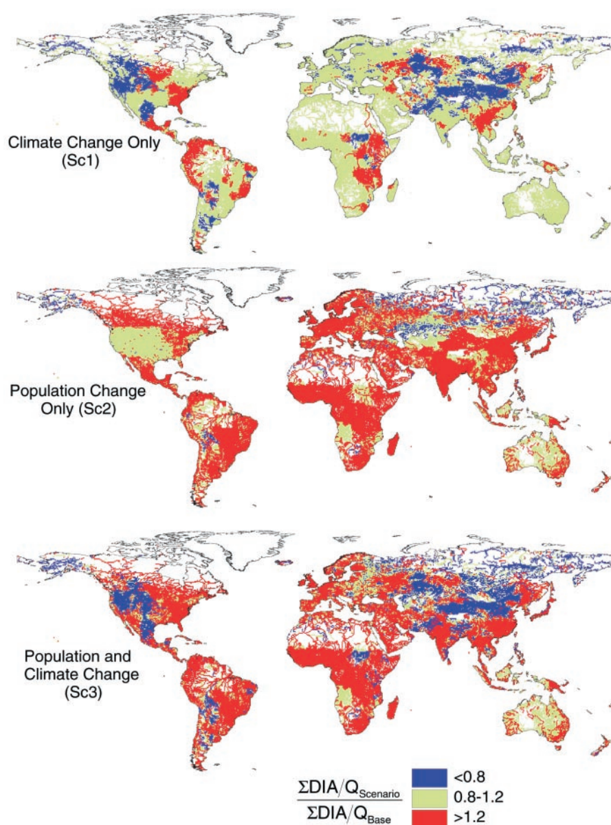
Fig. 3. Maps of the change in water reuse index ( \Sigma\text{DIA}/Q ) predicted by the CGCM1/WBM model configuration under Sc1 (climate change alone), Sc2 (population and economic development only), and Sc3 (both effects). Changes in the ratio of scenario-specific \Sigma\text{DIA}/Q ( \Sigma\text{DIA}/Q_{\text{Scenario}} ) relative to contemporary ( \Sigma\text{DIA}/Q_{\text{Base}} ) conditions are shown. A threshold of \pm 20\% is used to highlight areas of substantial change.
