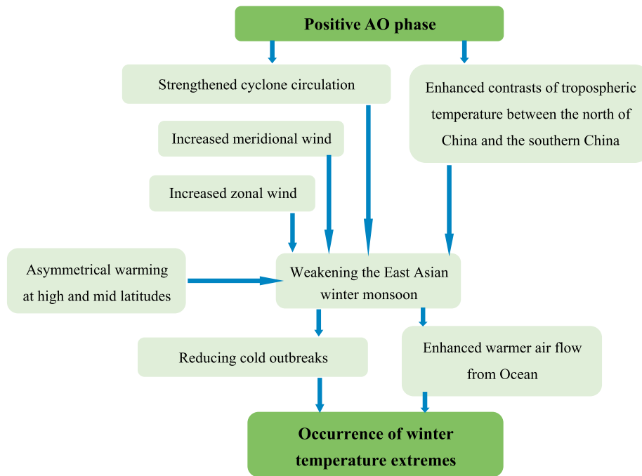
Figure 10. Possible causes of winter temperature extremes in China.
