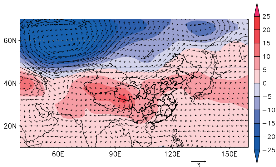
Figure 5. Differences (positive minus negative winter AO years) of mean geopotential height and wind field ( \text{m s}^{-1} ) at 850 hPa during 1961–2003.
