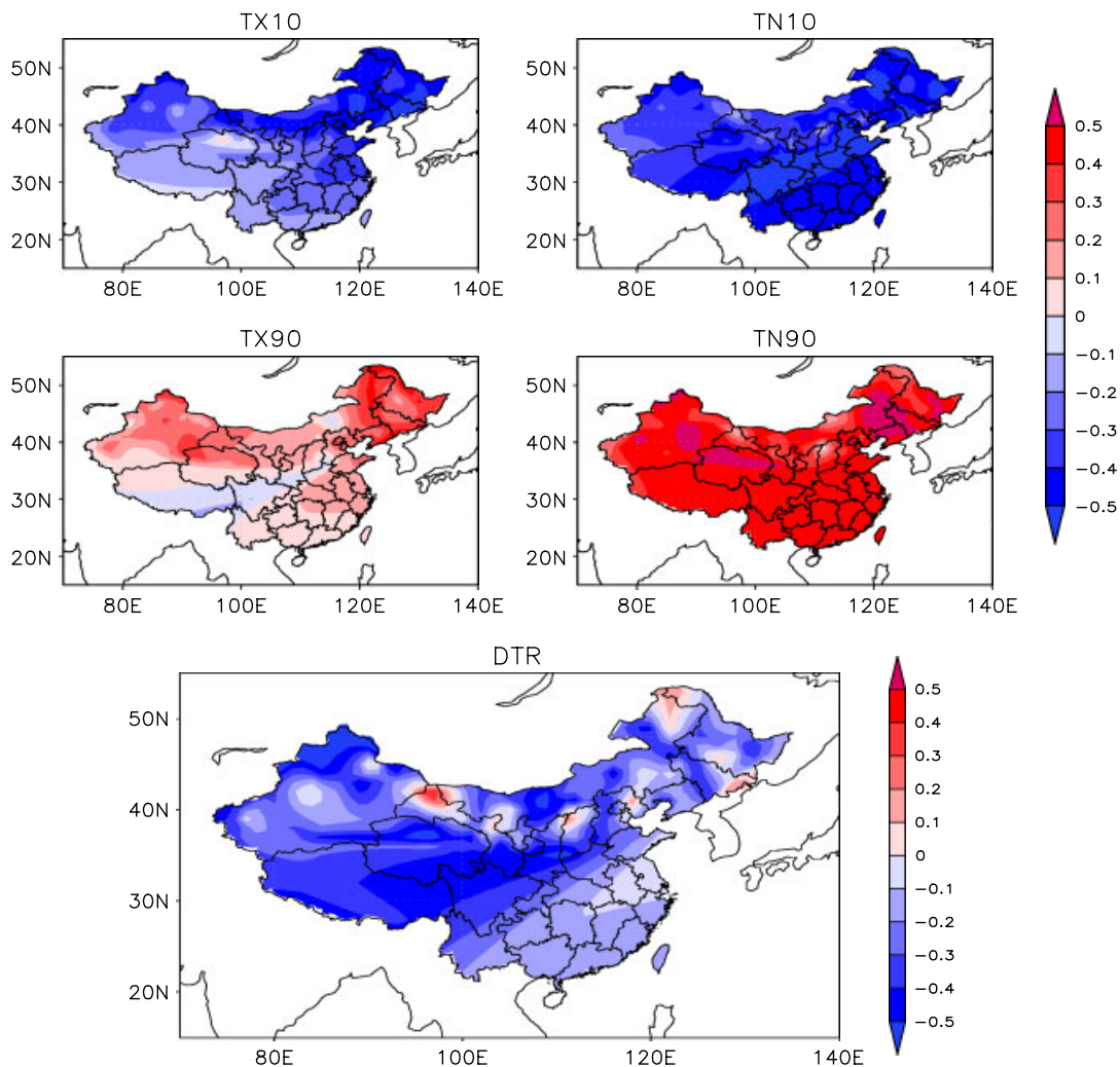
Figure 2. Spatial correlation coefficients between winter temperature indices (TX10, TN10, TX90, TN90 and DTR) and winter AO index during 1961–2003 in China.
