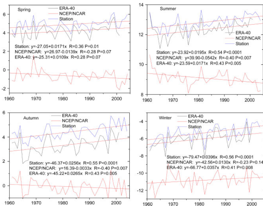
Figure 3. Average regional trends for surface stations, NCEP/NCAR and ERA-40 during 1961–2004 on a seasonal basis. Other is same as Figure 2. This figure is available in colour online at wileyonlinelibrary.com/journal/joc
