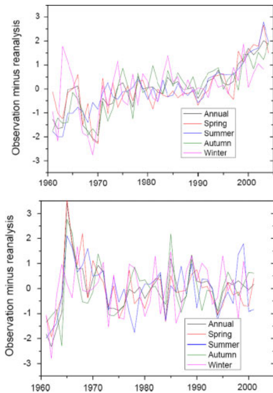
Figure 6. The anomaly of standard deviation for observation minus reanalysis (OMR) for NCEP/NCAR (top plot) and ERA-40 (bottom plot) during 1961–2004 and 1961–2001, respectively. This figure is available in colour online at wileyonlinelibrary.com/journal/joc
