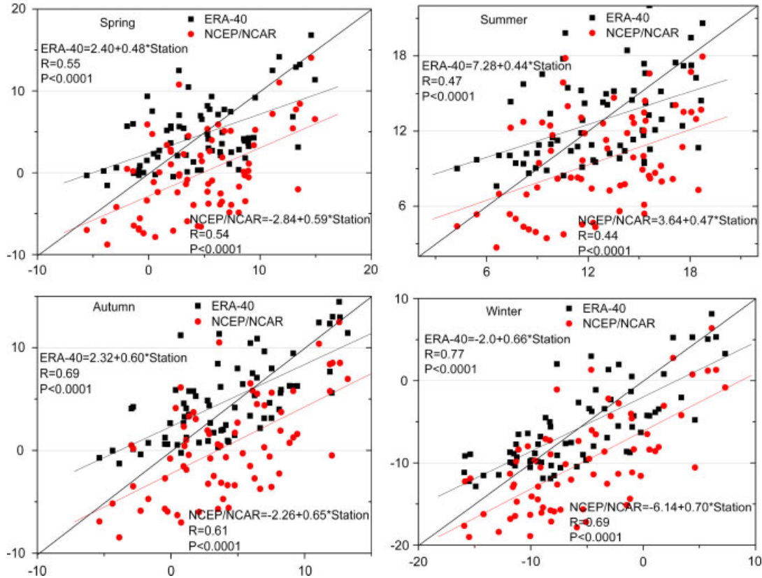
Figure 2. Comparison of temperature of surface stations during 1961–2004 with temperature from NCEP/NCAR and ERA-40 reanalysis data on a seasonal basis. The straight lines are linear fits, and R stands for correlation coefficients and P for statistical significance. This figure is available in colour online at wileyonlinelibrary.com/journal/joc
