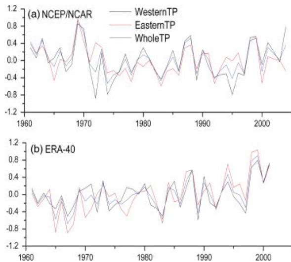
Figure 5. Average annual regional trends for the whole TP, eastern TP and western TP based on NCEP/NCAR (a) and ERA-40 (b) during 1961–2004 and 1961–2001, respectively. This figure is available in colour online at wileyonlinelibrary.com/journal/joc
