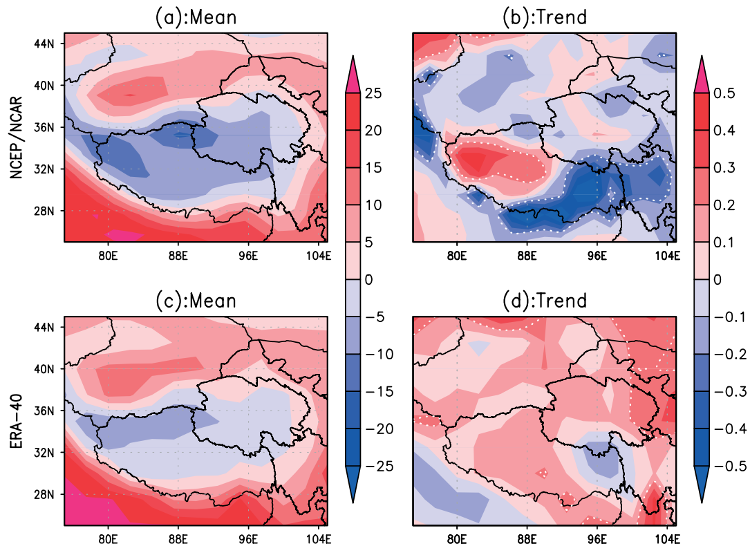
Figure 4. Spatial distribution of annual mean temperature (left plot, unit: °C/decade) and temperature trend magnitudes (right plot, unit: °C/decade) based on NCEP/NCAR and ERA-40 during 1961–2004 and 1961–2001, respectively. This figure is available in colour online at wileyonlinelibrary.com/journal/joc
