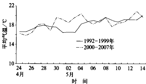
图 1 1999 年前后各 8 年“五一”期间逐日平均气温 Fig 1 Daily average temperature during the vacations of Internation Labor Day in the 8 years before and after 1999
